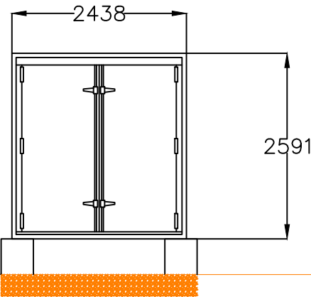
Spares container Side view
