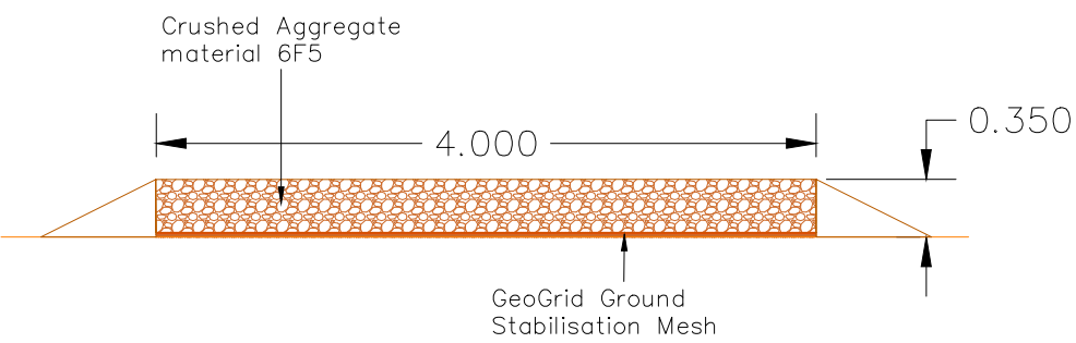
Alternative No-dig (Non-intrusive) access track
