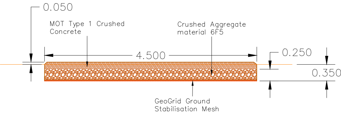
Typical DNO access track cross section
