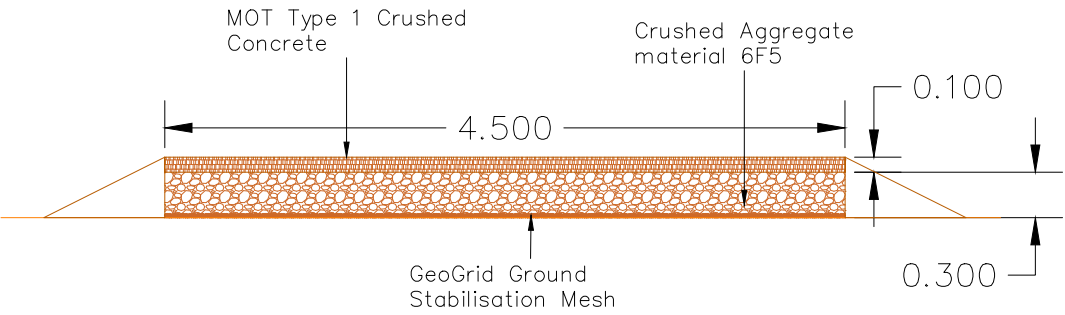
Alternative No-dig (Non-intrusive) DNO access track
