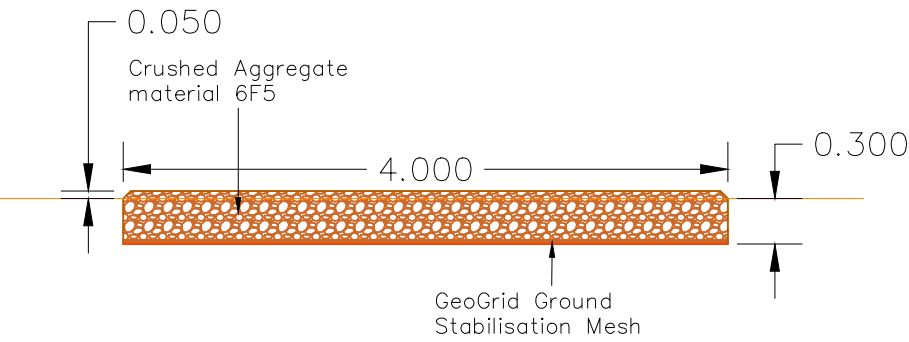
Typical access track cross section
