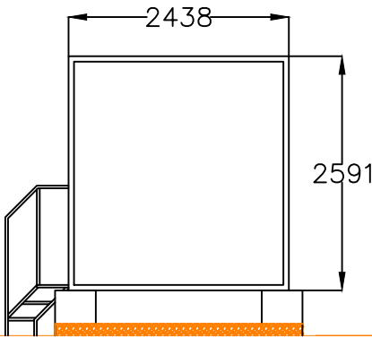
Customer switchgear Side view
