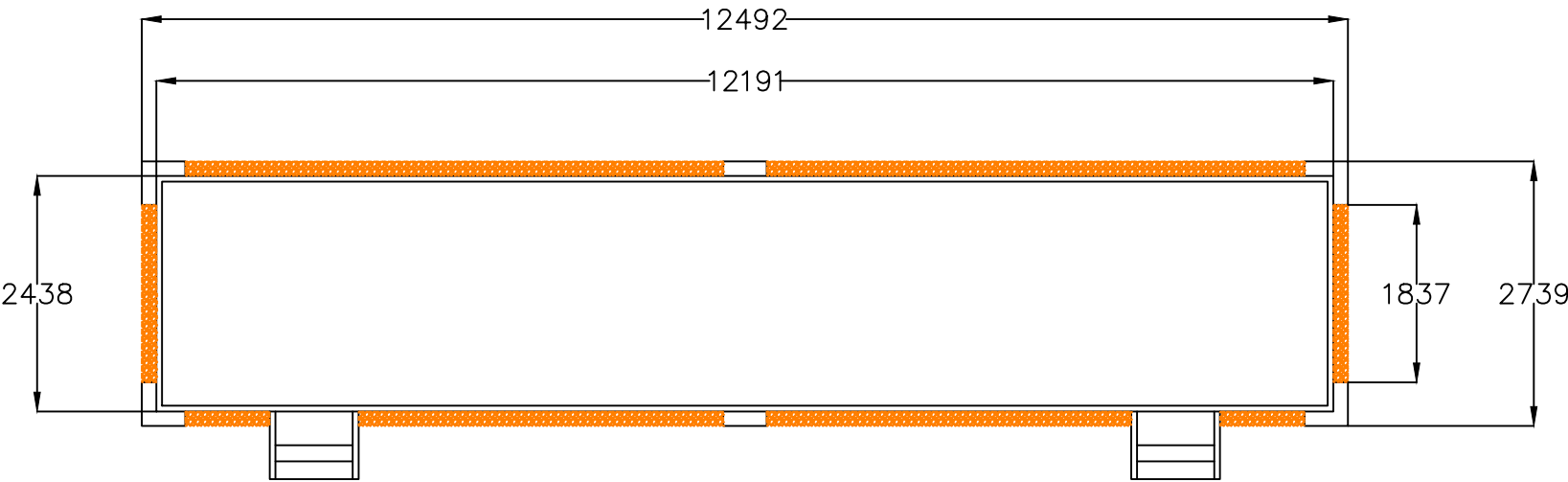
Customer switchgear Top view
