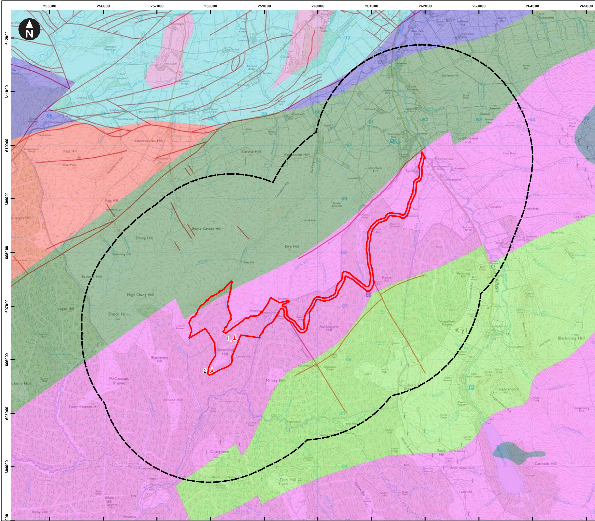
Figure 13.2 Bedrock geology
