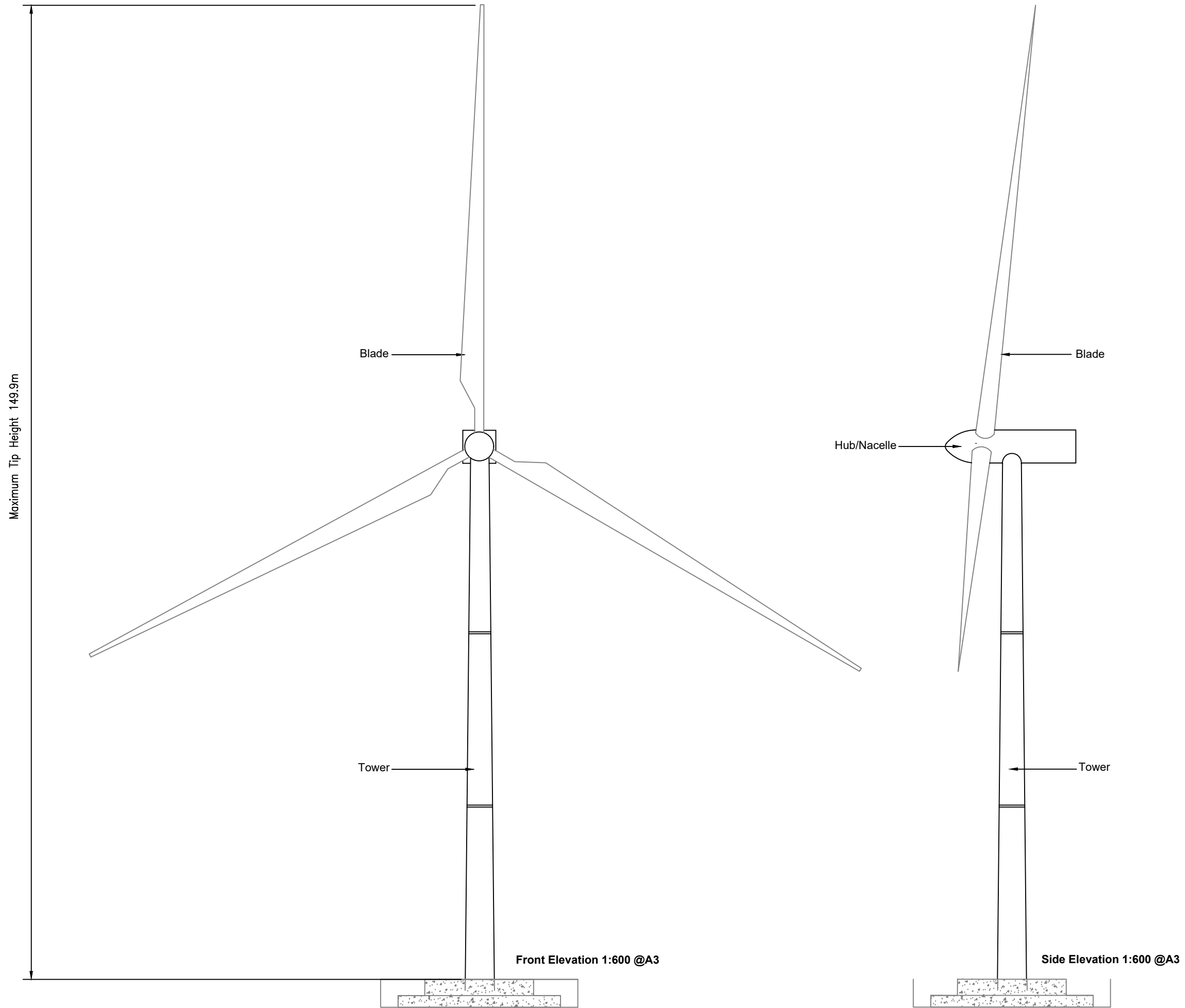
Figure 3.2 Typical wind turbine structure
