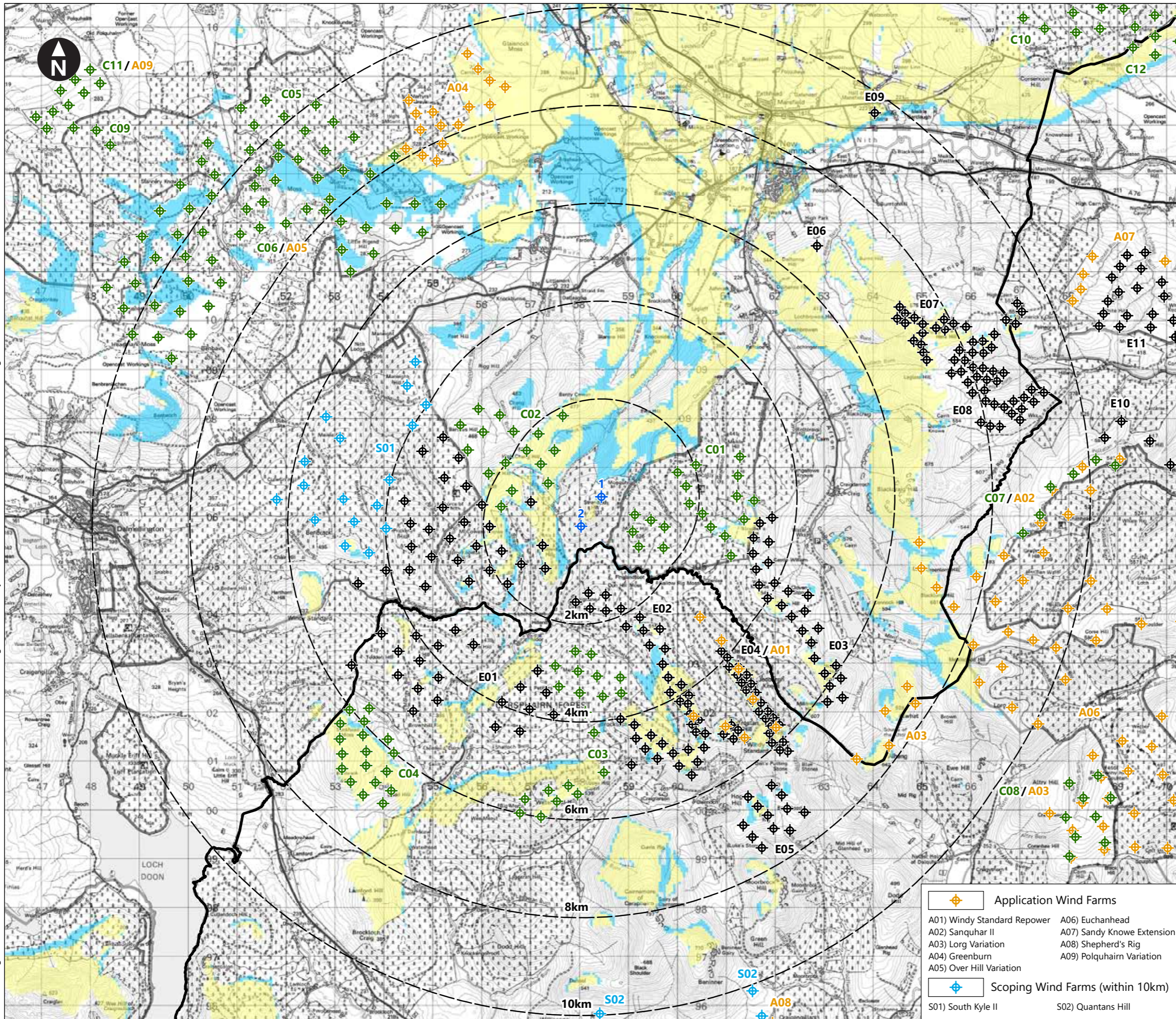
Figure 9.5 Zone of Theoretical Visibility (ZTV) to Hub Height (allowing for forestry) with Cumulative Wind Farms
