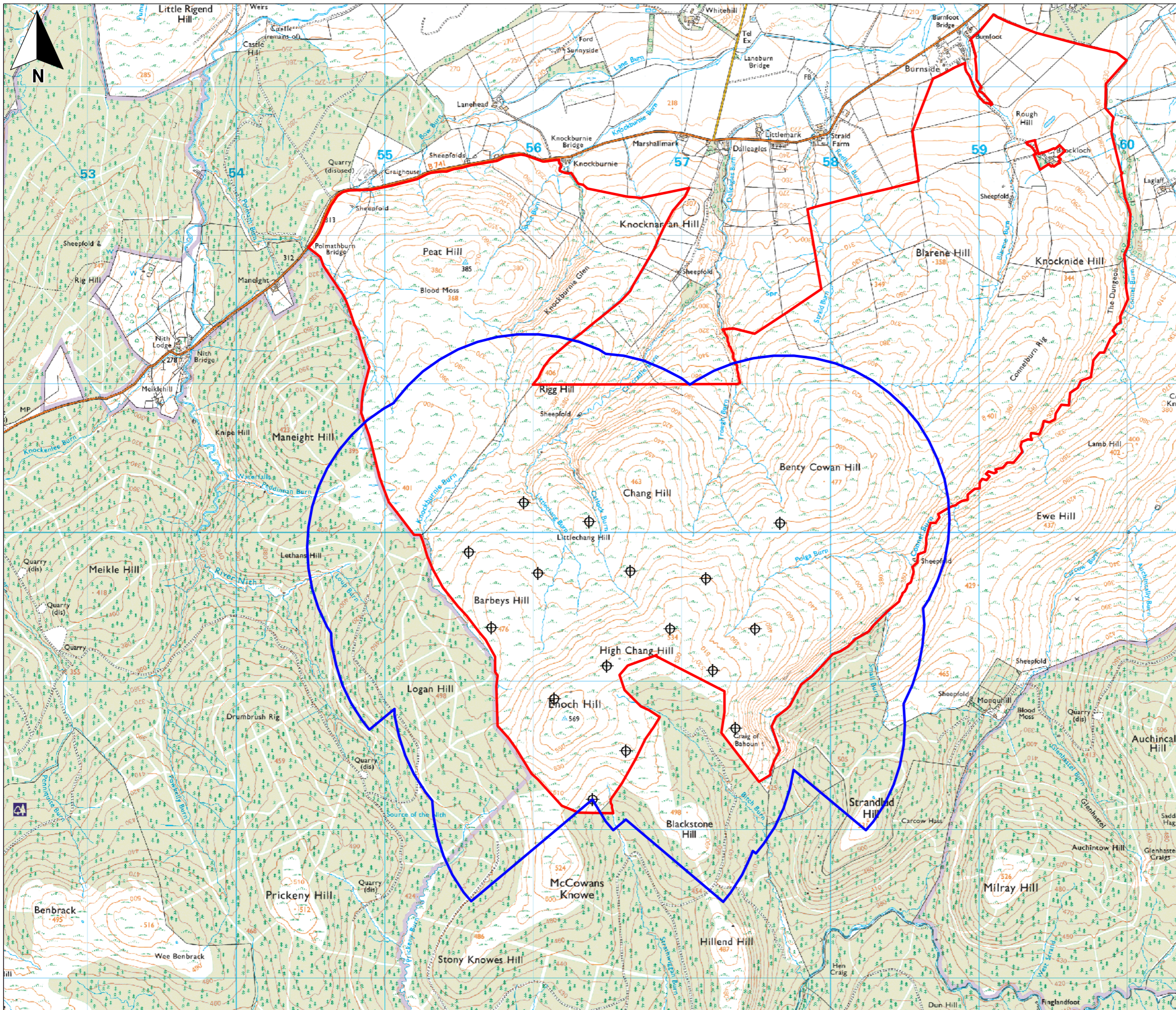
Figure 8.1 Shadow Flicker Study Area
