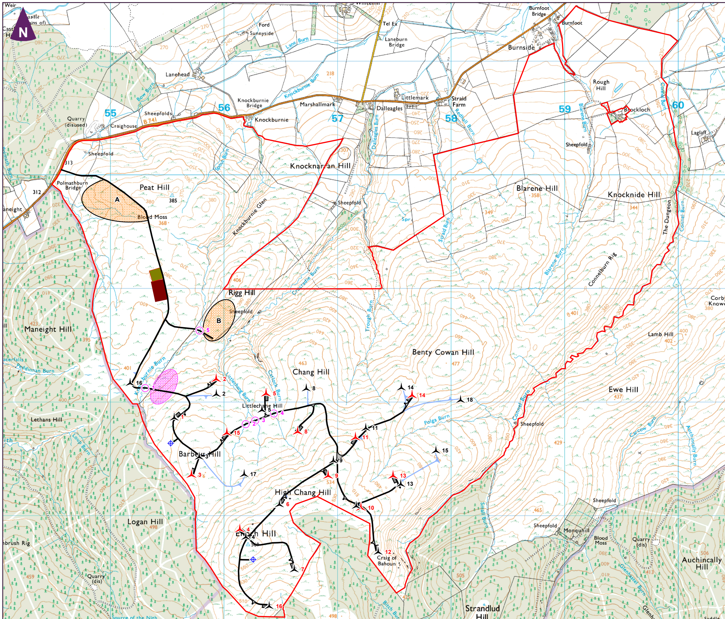
Figure 1.2 Revised Site Layout Compared to September 2015 Application Layout
