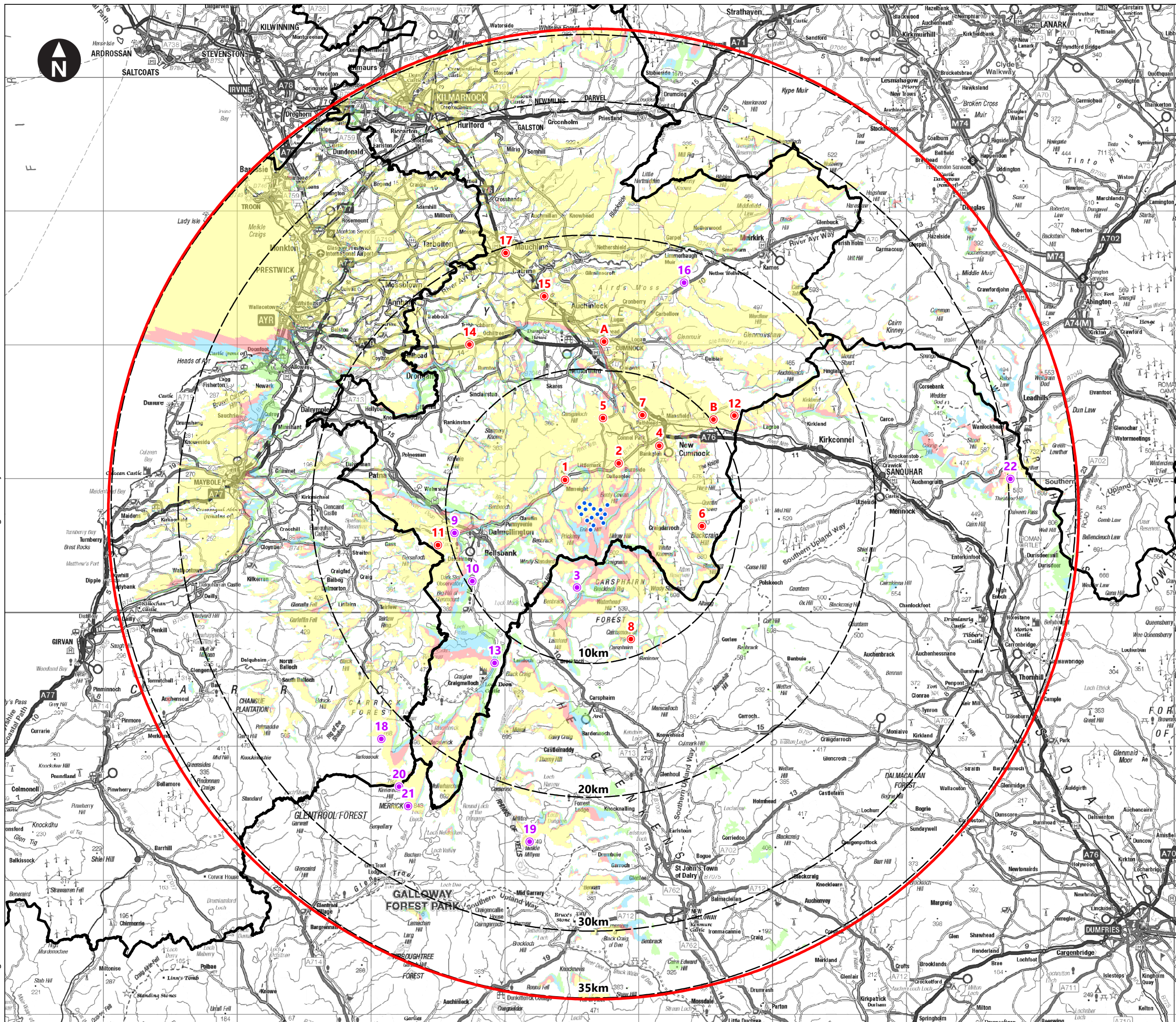
Figure V9.2 Zone of Theoretical Visibility (ZTV) to Blade Tip with Viewpoint Locations
