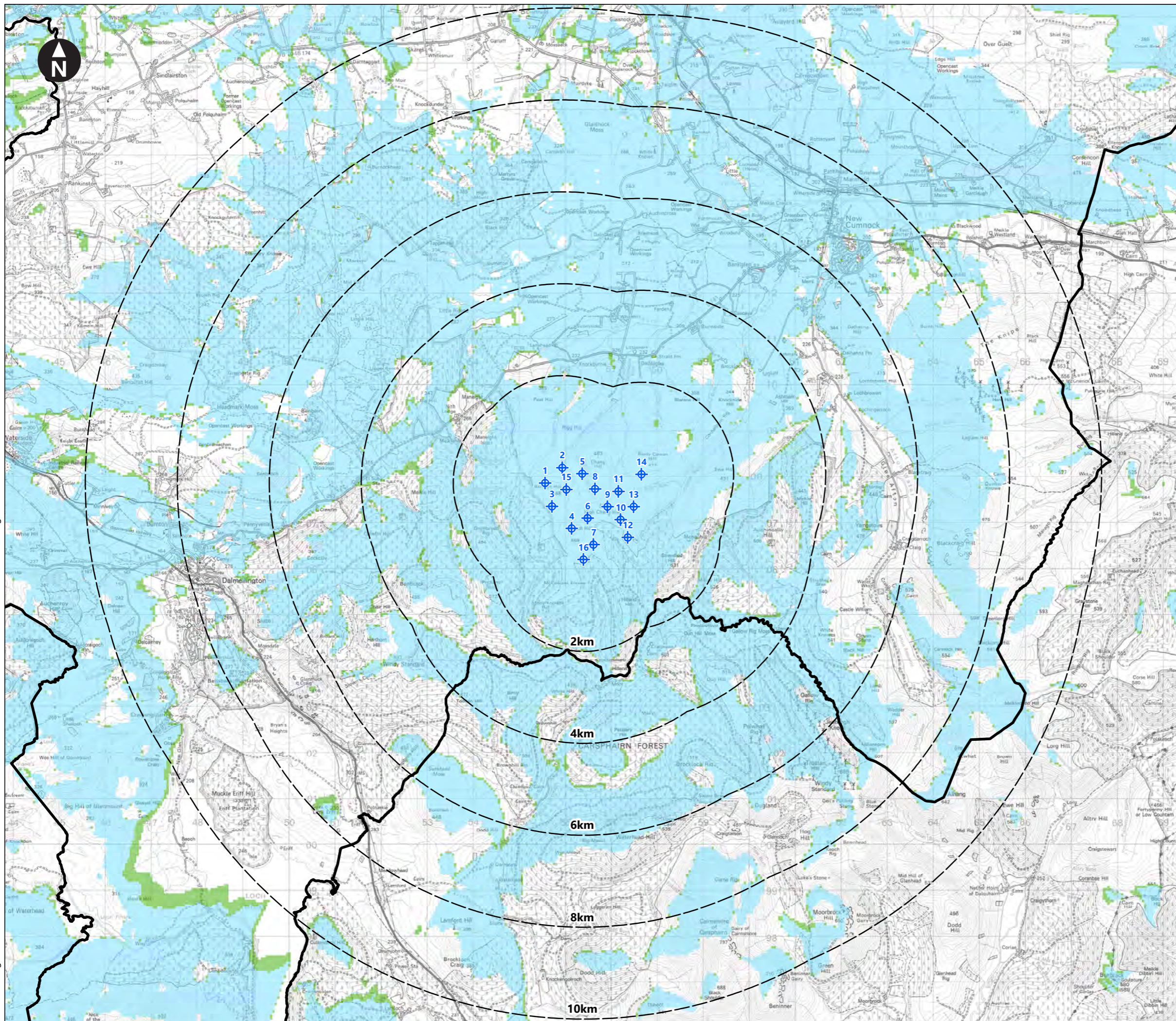
Figure V9.C Comparative ZTV to Blade Tip (10km)
